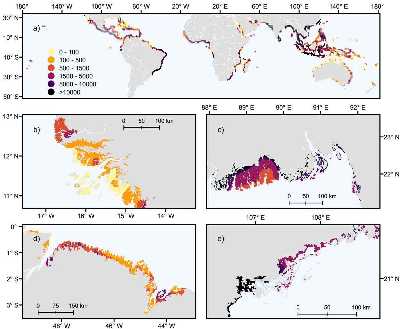
Fig. 3. Global map of small scale fishing intensity (fisher days \text{km}^{-2} \text{year}^{-1} ) within mangrove ecosystems, a) maximum fishing intensity within 1^\circ cells, high intensity areas (resolution \text{km}^2 ) in b) Guinea-Bissau, c) the Sundarbans of Indian and Bangladesh and coast of Myanmar, d) deltaic coast of Brazil, and e) the coast of Vietnam and China.
