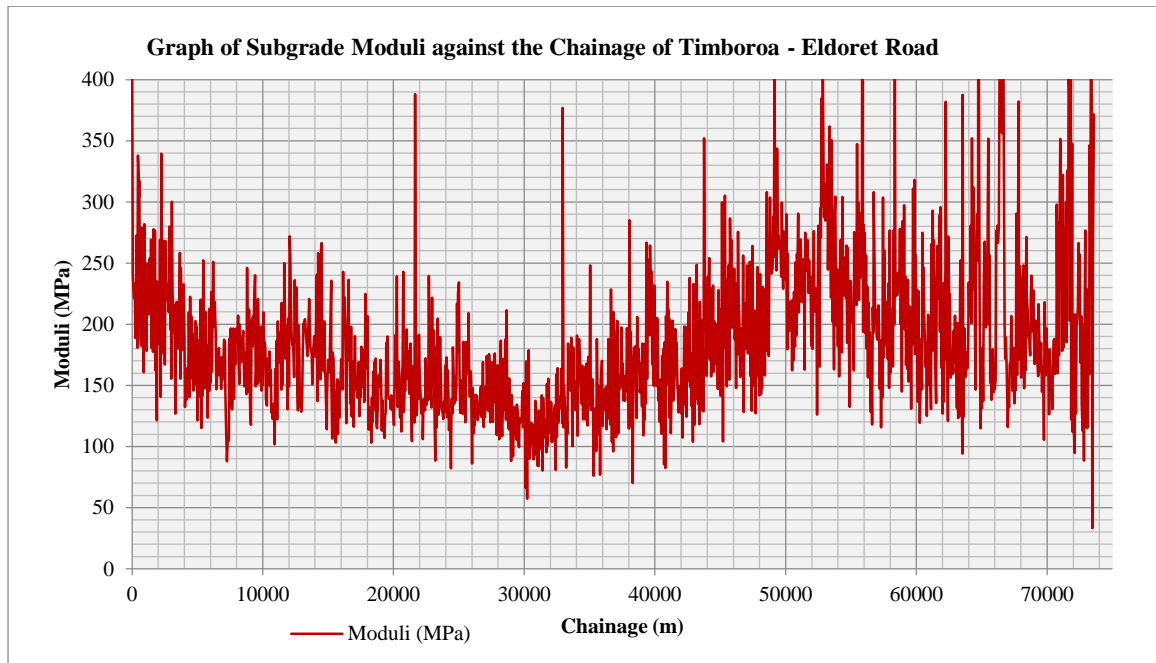
Figure 2: Moduli of subgrade layer along Timboroa – Eldoret section
