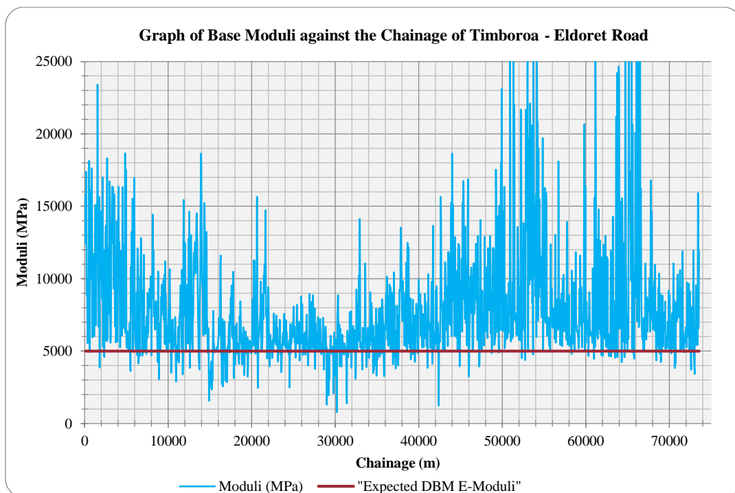
Figure 4: Moduli of base layer along Timboroa – Eldoret section
