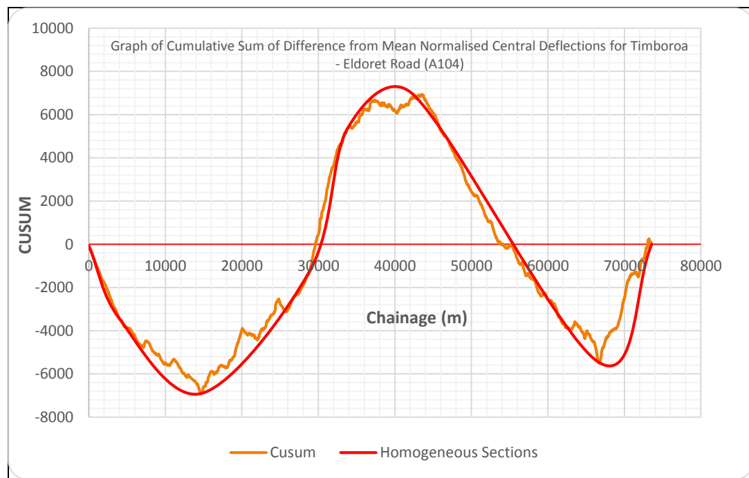
Figure 9: Plot of Cumulative Sum of Mean Normalized Central Deflections
