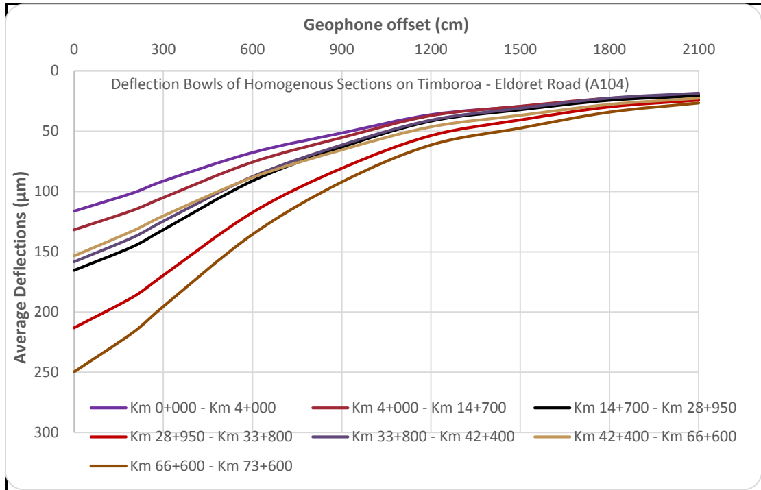
Figure 10: Deflection bowls of Homogenous sections
