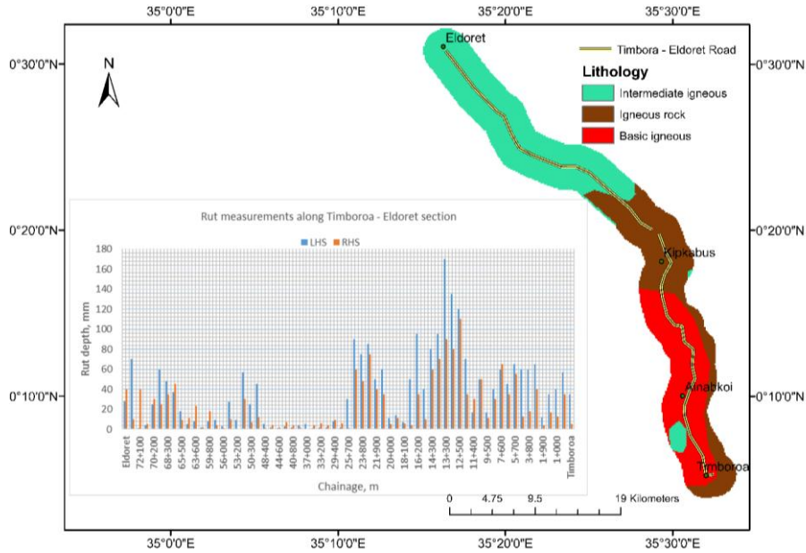
Figure 7: Correlation between Rut depth and Lithology
