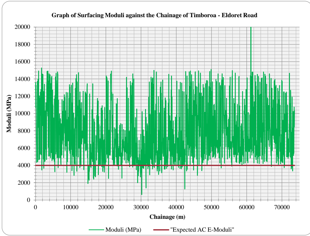
Figure 5: Moduli of Surfacing along Timboroa – Eldoret
