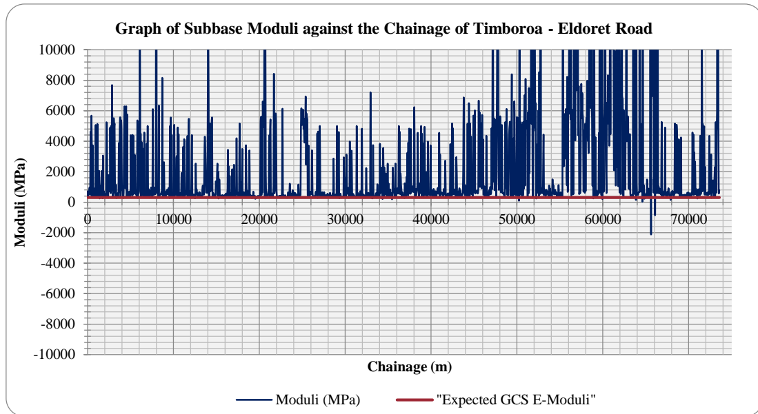
Figure 3: Moduli of subbase layer along Timboroa – Eldoret section
